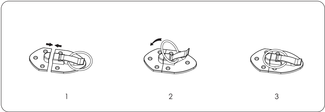
Outer buckle installation method
